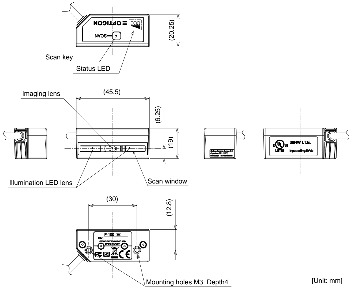
Figure 26: Mechanical Drawing
