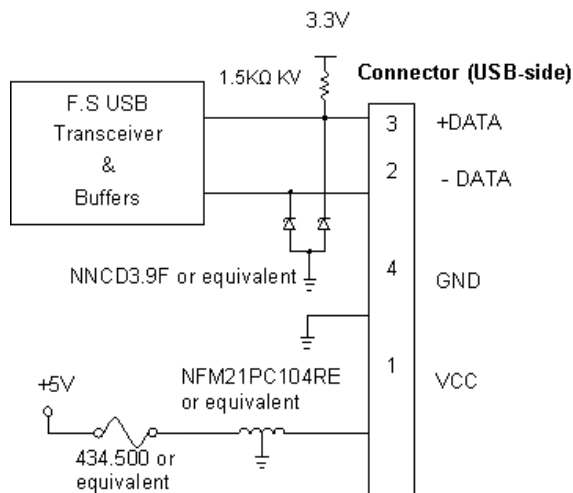
Figure 20: Interface circuit
