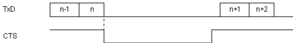
Figure 12: Signal timing
