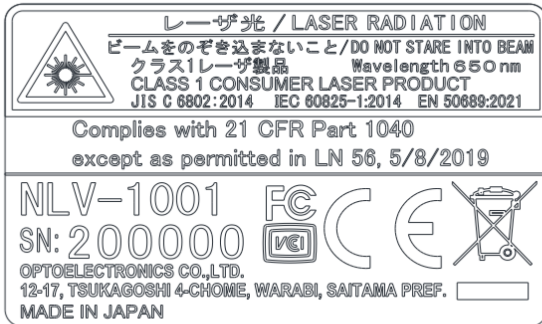
Figure 26: Serial number diagram
