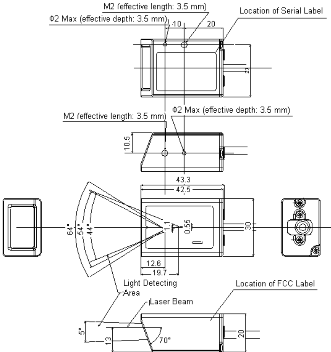
Figure 29: Mechanical drawing
