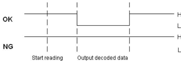
Figure 16: Good read (synchronous)
