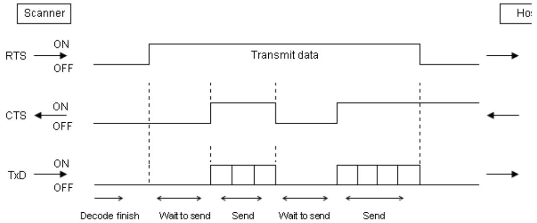
Figure 13: Handshaking—modem
