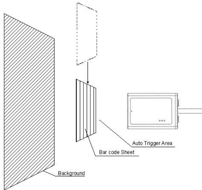
Figure 28: Auto trigger detection area
