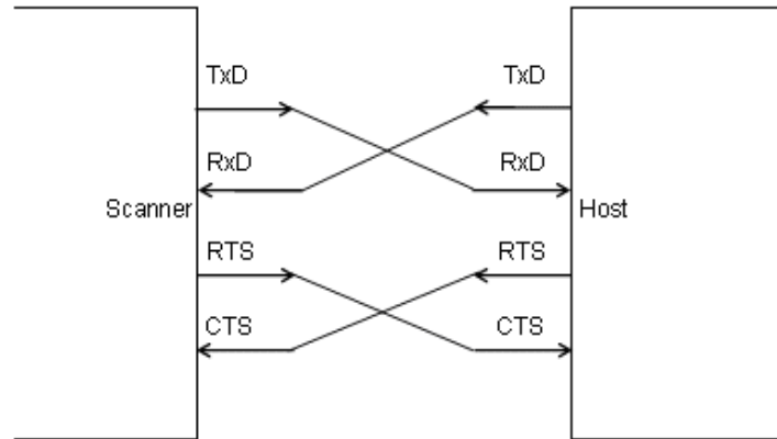
Figure 10: Busy/Ready communication
